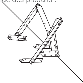
FIGURE A, ROOF MOUNT FIGURA A, MONTAJE AL TEJADO FIGURE A, MONTAGE AU TOIT
